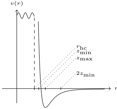
FIGURE 1. A typical pair interaction potential with 0 \leq r_{\text{hc}} < z_{\text{min}} < z_{\text{max}} < 2z_{\text{min}} as specified in Assumption 1.
