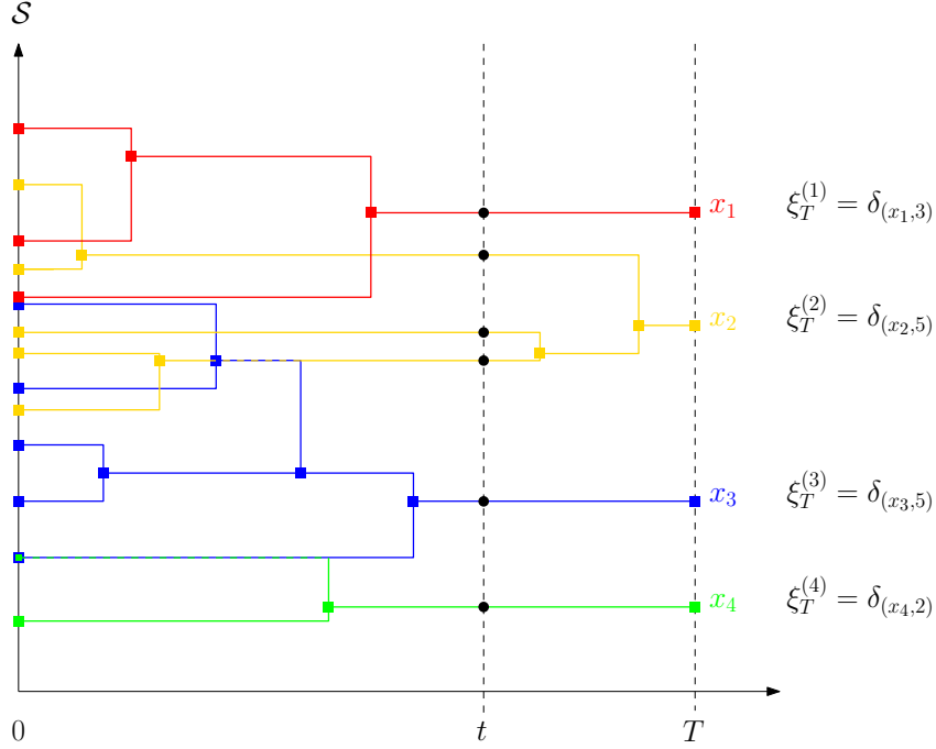
Fig 1: An illustration of the decomposition of (\Xi_t)_{t \in [0, T]} into four subprocesses (\xi_t^{(i)})_{t \in [0, T]} , i = 1, \dots, 4 , that are distinguished by their colour. The process (\Xi_t)_{t \in [0, T]} is started from 15 atoms at time 0 and ends up with 4 particles. However, each subprocess (\xi_t^{(i)})_{t \in [0, T]} , i = 1, \dots, 4 , ends in a single-particle configuration by definition. At time t , there are 6 particles with masses 3, 2, 1, 2, 5 and 2.
