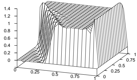
Fig. 4: Example 2, SUPG, N = 20 .
