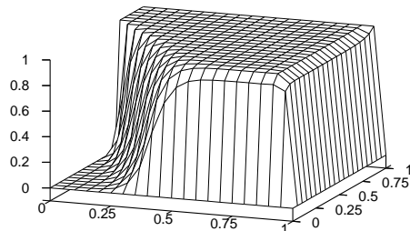
Fig. 13: Example 2, CG, N = 20 .
