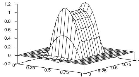
Fig. 6: Example 3, SUPG, N = 20 .
