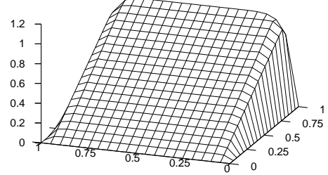
Fig. 8: Example 1, C_{mod}, C = 0.6, N = 20 .
