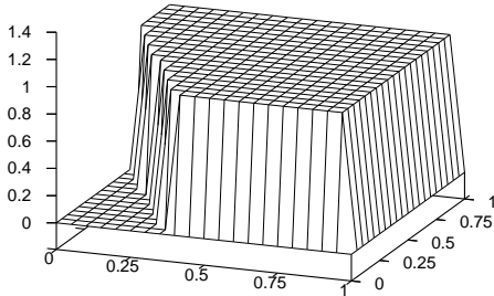
Fig. 3: Example 2, solution u .
