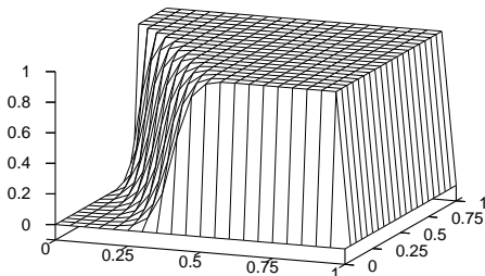
Fig. 12: Example 2, IMH, N = 20 .
