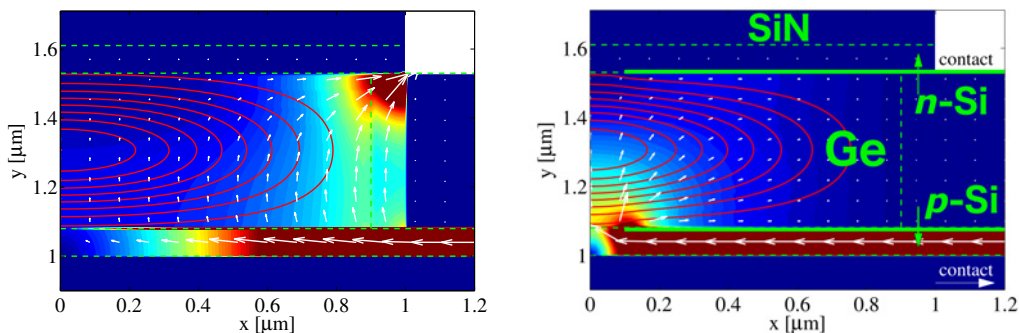
Fig. 7: Hole current for left: standard device and right: aperture device above threshold. Red lines indicate the isolines of \Theta^2 , whereas the white arrows and the colored background show the direction and magnitude of (the current) j_p = -\mu_p p \nabla \phi_p .
