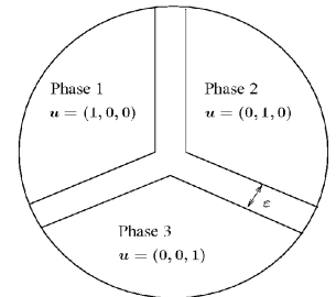
Fig. 7: Phase field model with three phases, which are separated by a diffuse interface of thickness \varepsilon
