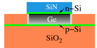
Fig. 5: Cross section through standard Ge heterostructure similar to Fig. 1
