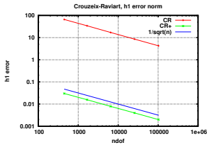
Fig. 2: Comparison of accuracy between the 1973 Crouzeix–Raviart (CR) mixed finite element method versus the new pressure-robust Crouzeix–Raviart element (CR + ) [3] for an incompressible Stokes problem with \nu = 10^{-3} . Comparison of H^1 error. The new pressure-robust Crouzeix–Raviart element is about ten refinement levels more accurate, which is a computational speedup by roughly a factor of 10^6 .
