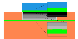
Fig. 6: Cross section through aperture Ge heterostructure
