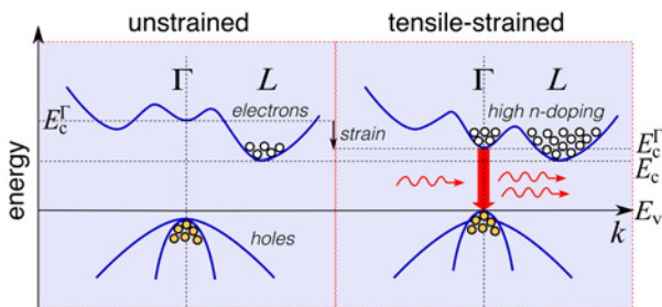
Fig. 2: Schematic Ge band structure showing the occupation of electrons and holes in the conduction and valence band. The combined effect of tensile strain and n -doping resulting in an increase of stimulated emission by reducing the direct band gap E_c^\Gamma - E_v (strain) and by filling the \Gamma -band (doping)
