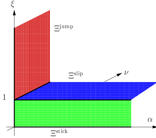
Figure 3.1: The set \Xi = \Xi^{\text{stick}} \cup \Xi^{\text{slip}} \cup \Xi^{\text{jump}}
