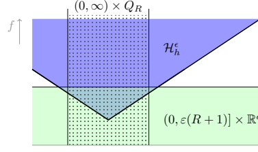
FIG 2. Illustration (0, \infty) \times Q_R \subset \mathcal{H}_h^\varepsilon \cup (0, \varepsilon(R+1)] \times \mathbb{R}^d .
