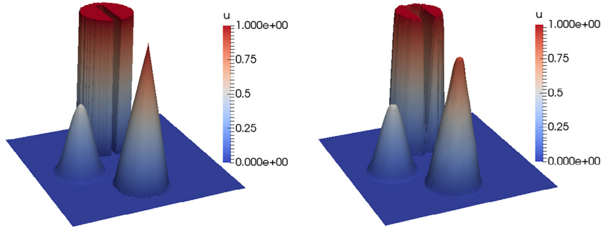
Fig. 1. Interpolated continuous initial condition (left) and solution at t = 6.28 for the FEM-FCT scheme (right).
