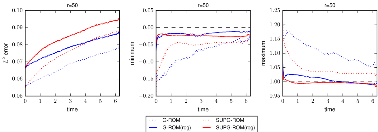
Fig. 4. Time evolution of the measures of interest for G-ROMs and SUPG-ROMs for r = 50 .
