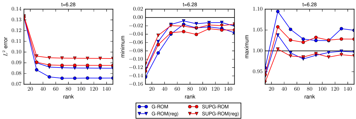
Fig. 3. Measures of interest at t = 6.28 .
