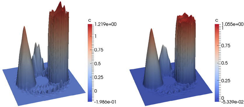
Fig. 2. Standard ROM initial condition (3) (left) and regularized ROM initial condition (5) (right) based on physically admissible snapshots from the FEM-FCT approach for r = 50 .
