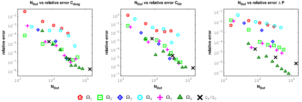
Fig. 4. Results for the two-dimensional flow around a cylinder for fourth order velocity and third order pressure.
