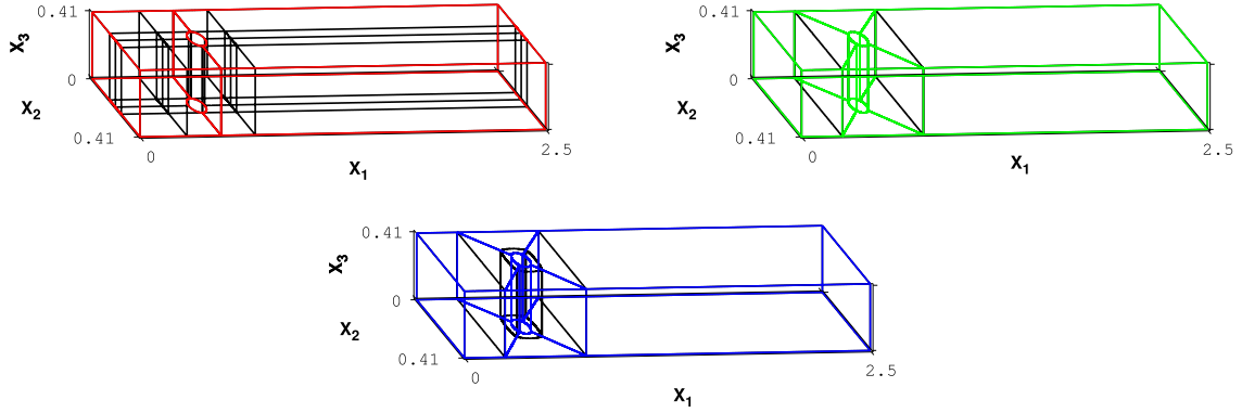
Fig. 5. Three-dimensional flow around a cylinder: Parametrizations of \Omega into patches: \Omega_3 , \Omega_5 , and \Omega_6 .
