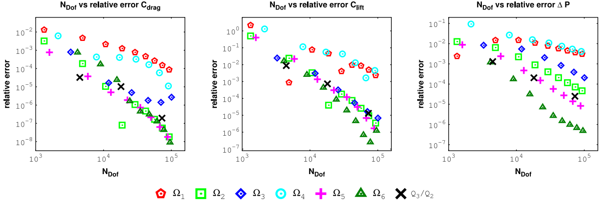
Fig. 3. Results for the two-dimensional flow around a cylinder for third order velocity and second order pressure.
