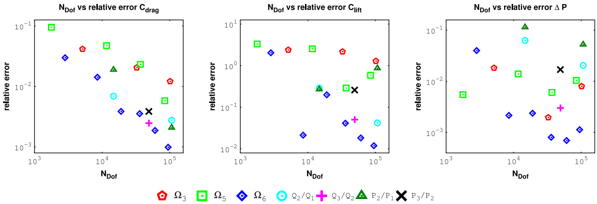
Fig. 6. Results for the three-dimensional flow around a cylinder for the IGA with third order velocity and second order pressure and for the finite element pairs Q_2/Q_1 , Q_3/Q_2 , P_2/P_1 , and P_3/P_2 .
