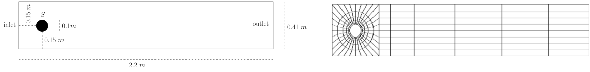
Fig. 1. Two-dimensional flow around a cylinder: Domain and coarsest finite element grid.
