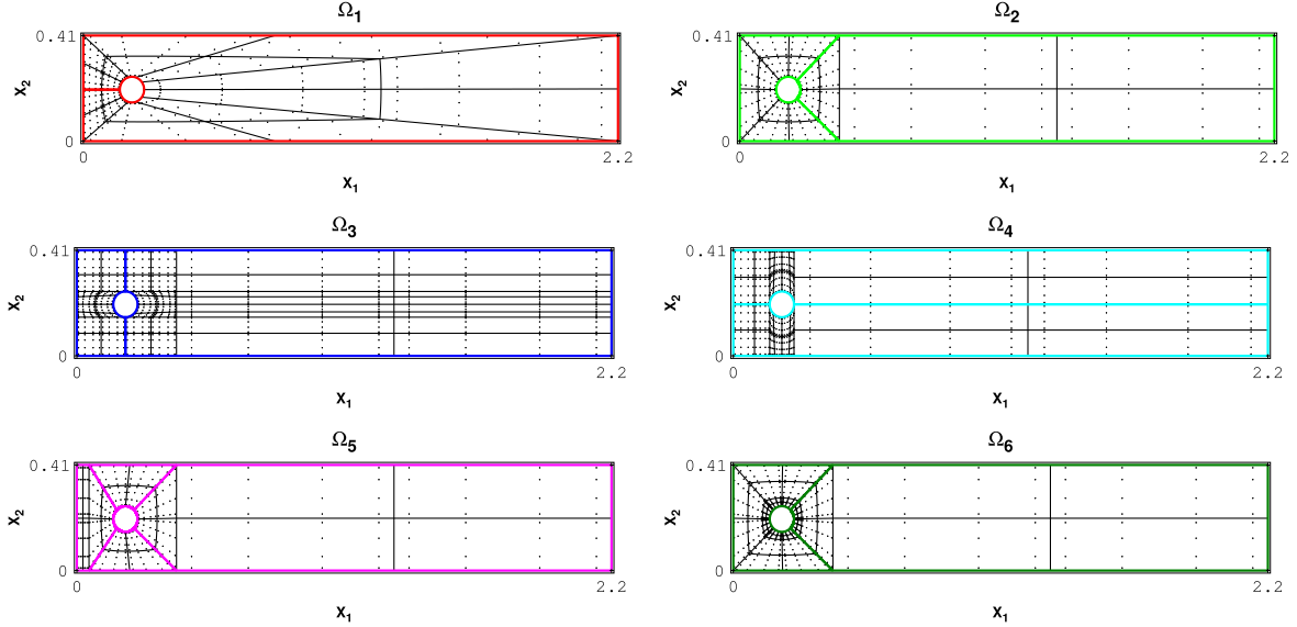
Fig. 2. Two-dimensional flow around a cylinder: Parametrizations of \Omega into patches: \Omega_1, \dots, \Omega_6 , left to right, top to bottom. The thick colored lines give the decomposition into patches, the thin lines the corresponding coarsest grids, and the dots the quadrature points. Note that \Omega_6 is more refined at the cylinder than \Omega_2 . (For interpretation of the references to color in this figure legend, the reader is referred to the web version of this article.)
