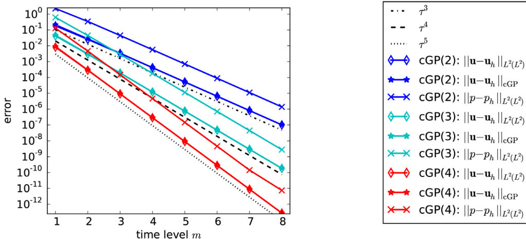
Fig. 2. Example 2: Convergence of various errors with respect to the time step, where the time step is given by \tau = 0.1 \cdot 2^{-m+1} .
