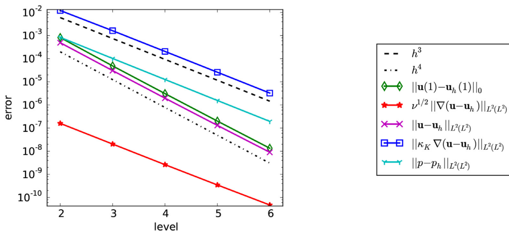
Fig. 1. Example 1: Convergence of various errors with respect to the spatial mesh width.
