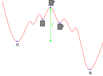
FIGURE 2. A nucleation path from \Xi_\Lambda to \oplus_\Lambda for Glauber dynamics. \Gamma in (1.10) is the minimal energy barrier the path has to overcome under the local variant of the Hamiltonian in (1.1).
