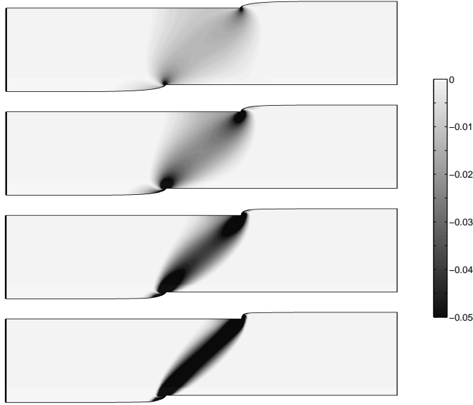
FIGURE 4. Displacement u_h and hardening variable \eta_h ( \sim |plastic strain|) for t = T and decreasing hardening parameter \varepsilon = 1, 1/4, 1/16, and 1/64 , showing how a diagonal slip-band becomes more and more pronounced. The underlying triangulation has 163 840 triangles, the discrete displacement is displayed magnified by a factor 4.
