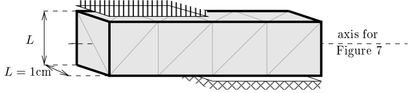
FIGURE 6. Geometry for the 3D example in Sect. 6.2
