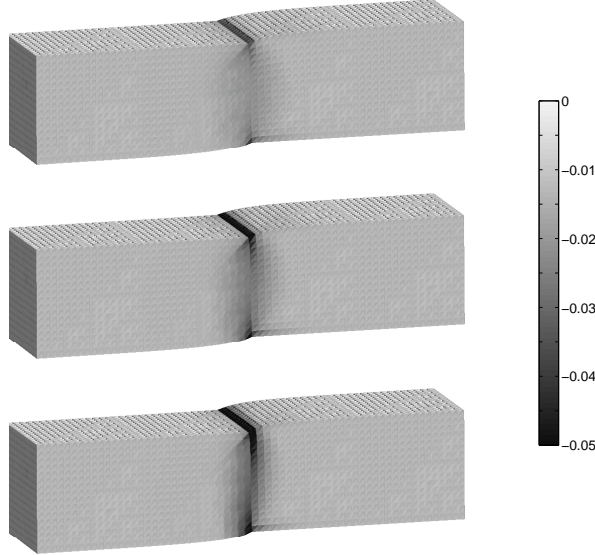
FIGURE 8. Displacement u_h and hardening variable \eta_h ( \sim |plastic strain|) for t = T and \varepsilon = 1, 1/4, and 1/16 , showing how a vertical slip-band becomes more and more pronounced. The underlying triangulation has 98 304 tetrahedra, the displacement is magnified by a factor 4.
