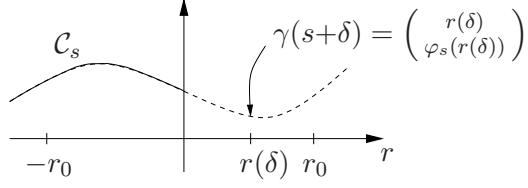
Figure 3.1: Local description of the crack \mathcal{C} via \varphi_s
